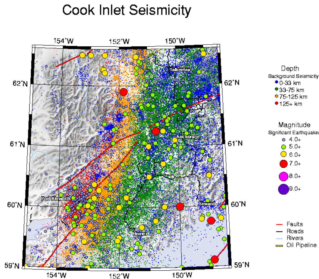
Figure 6 Homer Earthquake History
