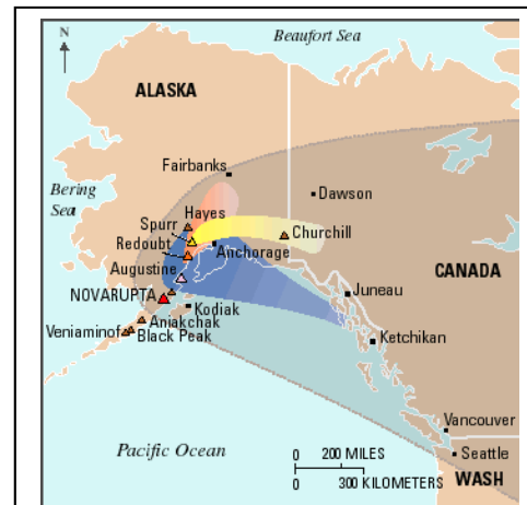
Figure 8: Novarupta ash fall compared to that from recent Alaskan eruptions.
