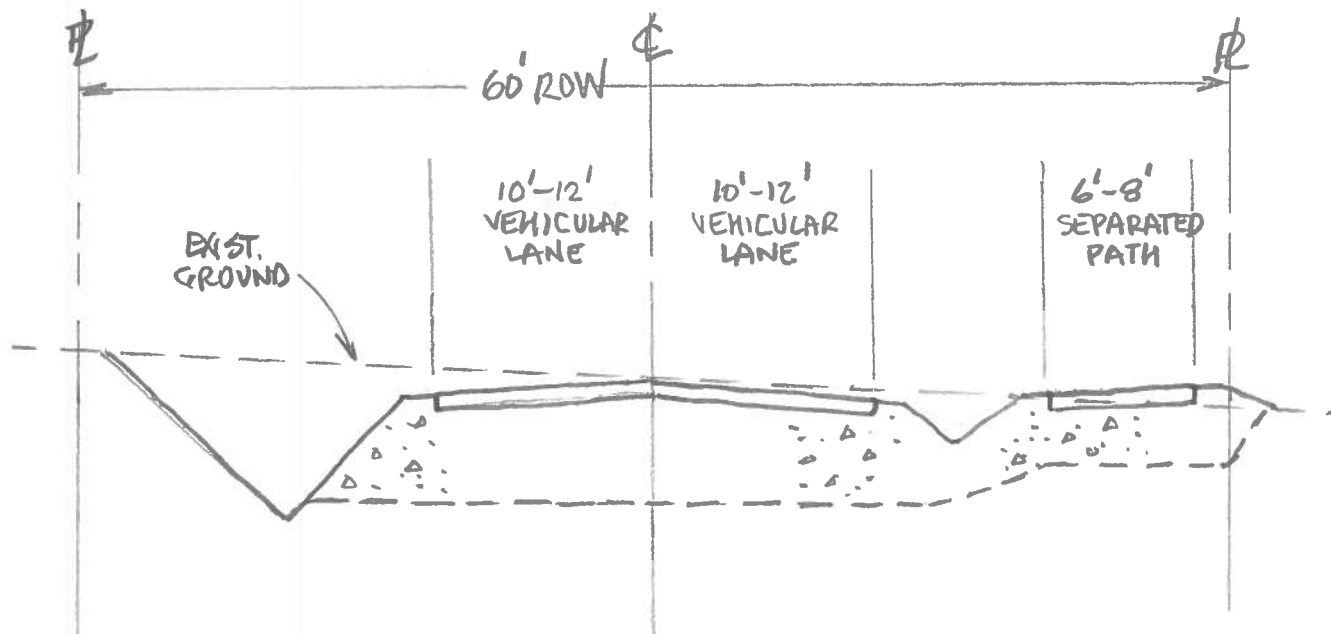
LEVEL 3 SINGLE SEPARATED PATHWAY
