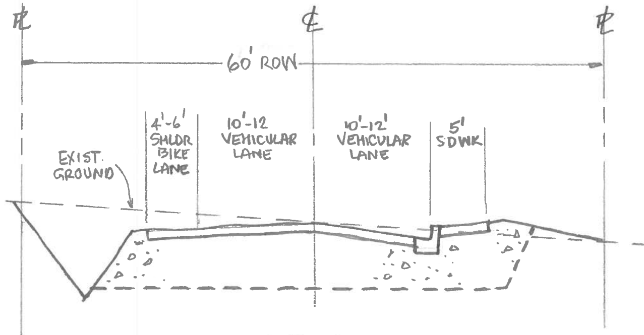
LEVEL 4 SIDEWALK/WIDENED PAVEMENT
