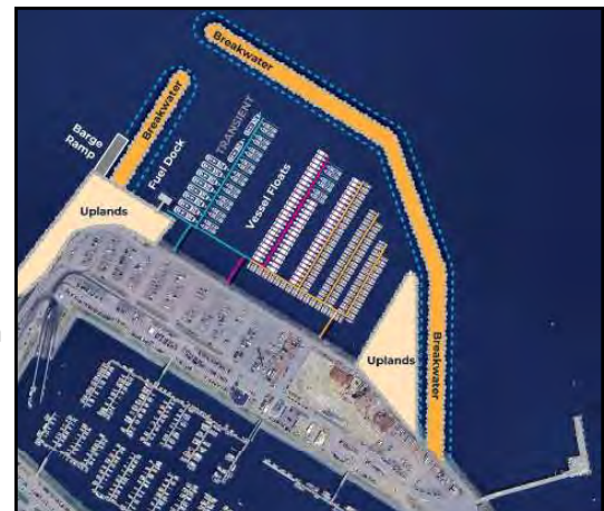
Port expansion adds a new basin with its own entrance adjacent to the existing Small Boat Harbor to relieve large vessel congestion in the small boat harbor, shown below.
